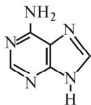
adenin (a)
